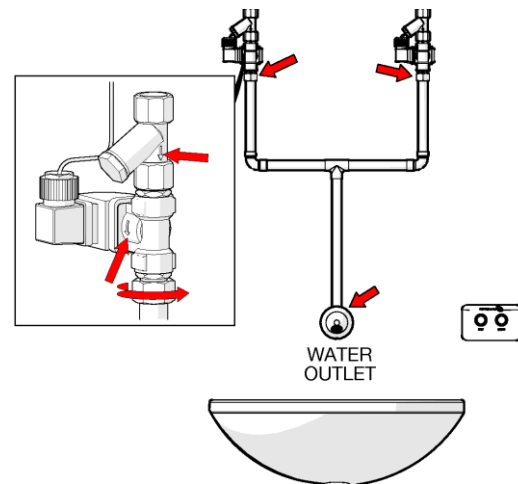
Typical Installation
